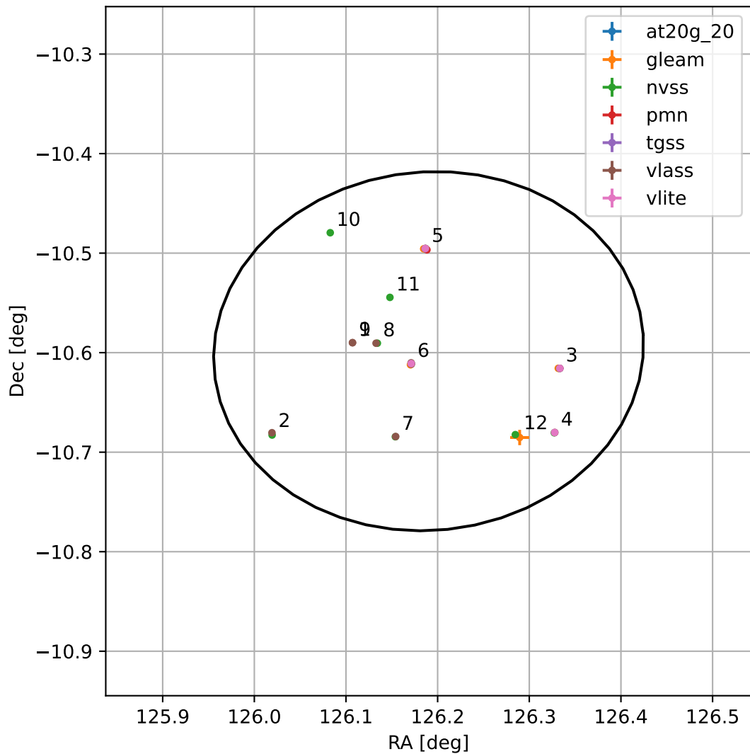
4FGL J0824.7-1035
