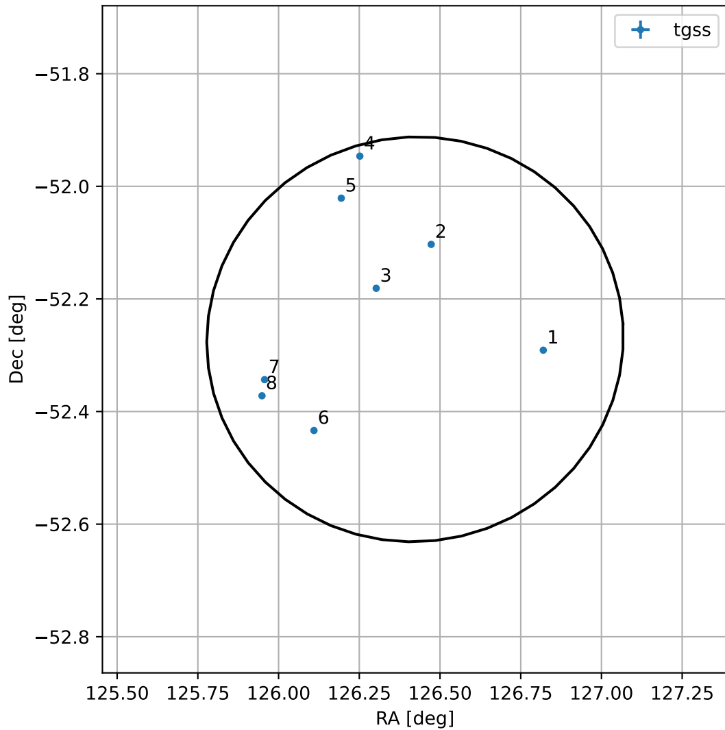
4FGL J0825.6-5216
