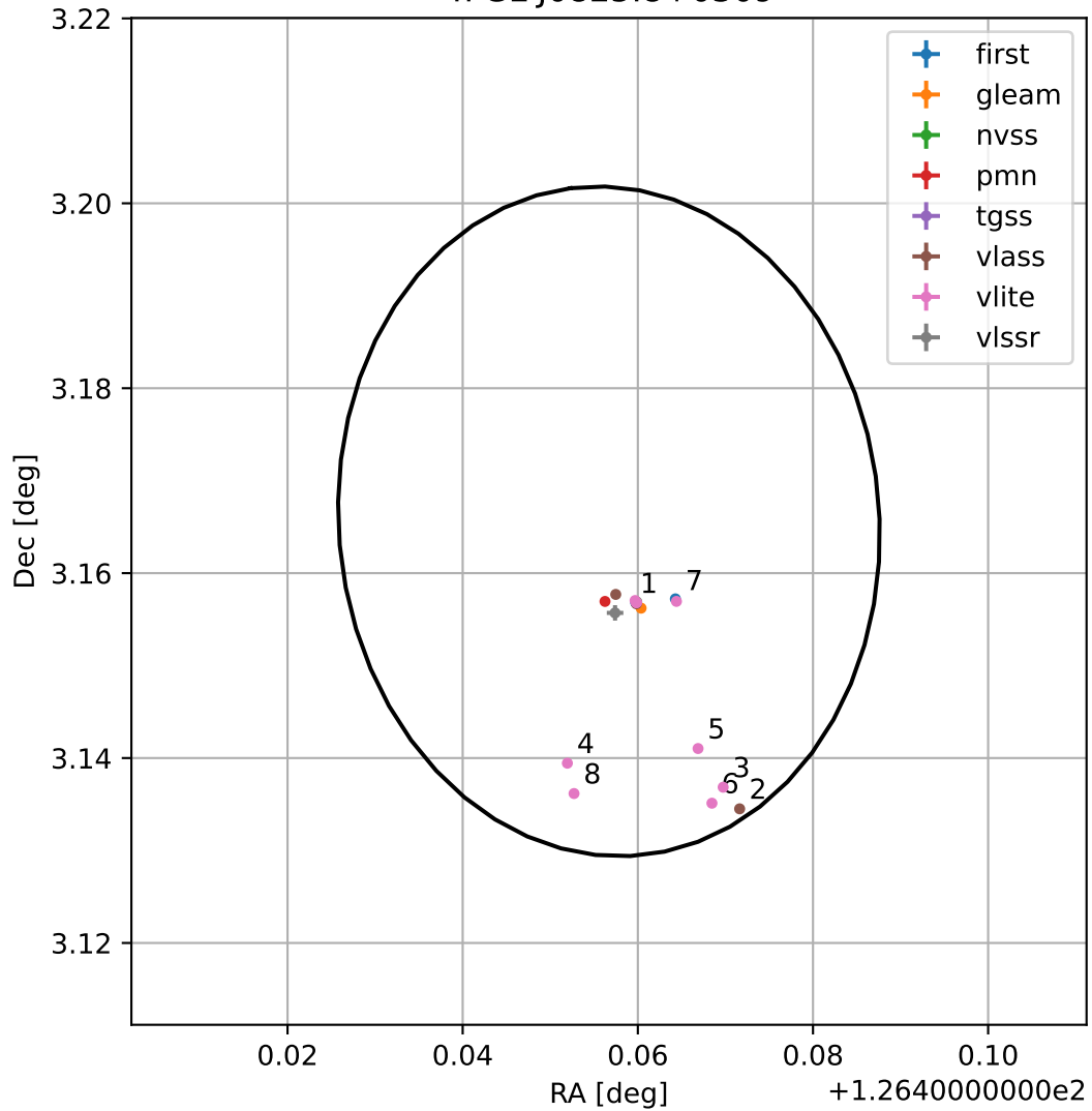
4FGL J0825.8+0309
