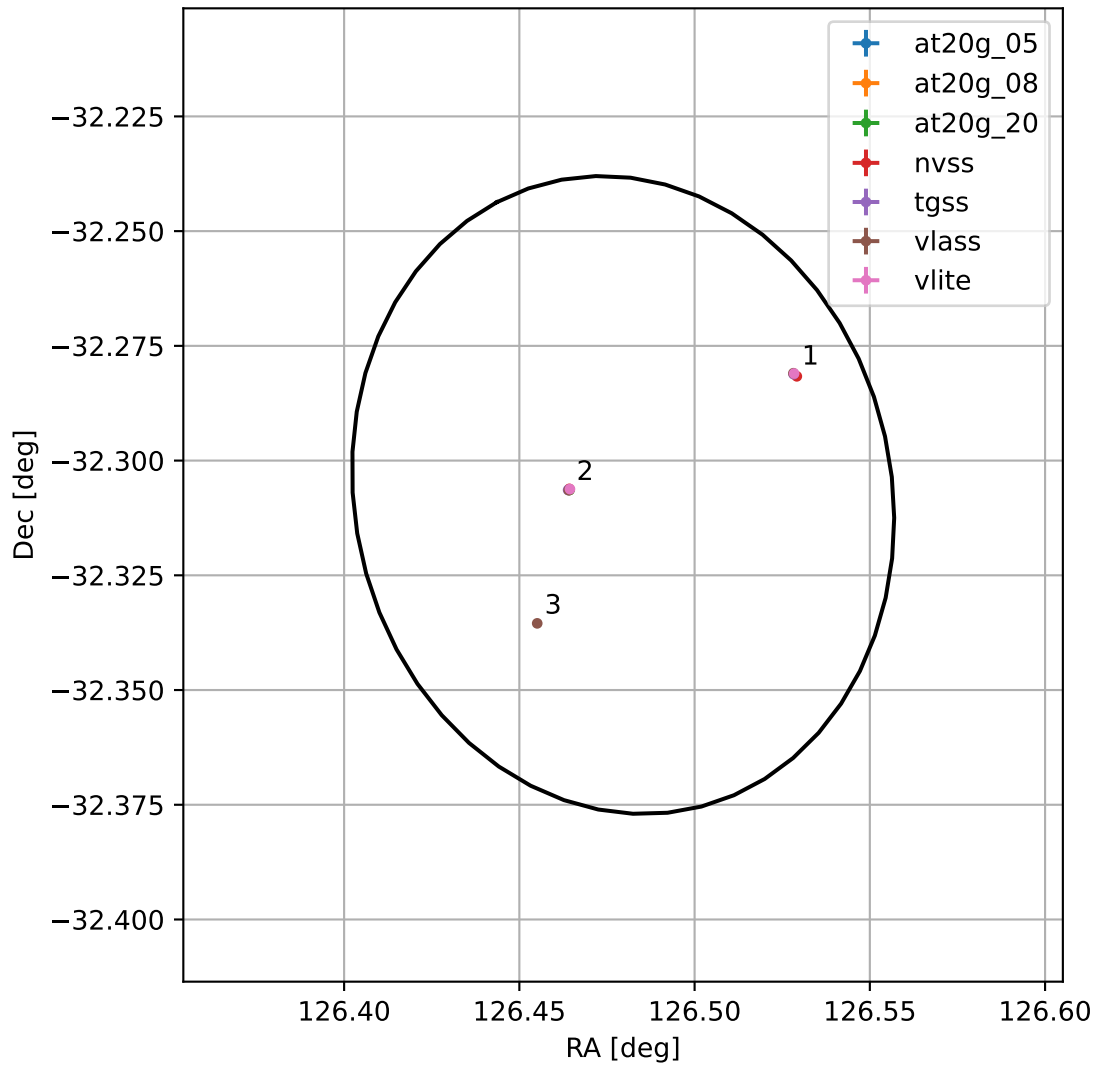
4FGL J0825.9-3218
