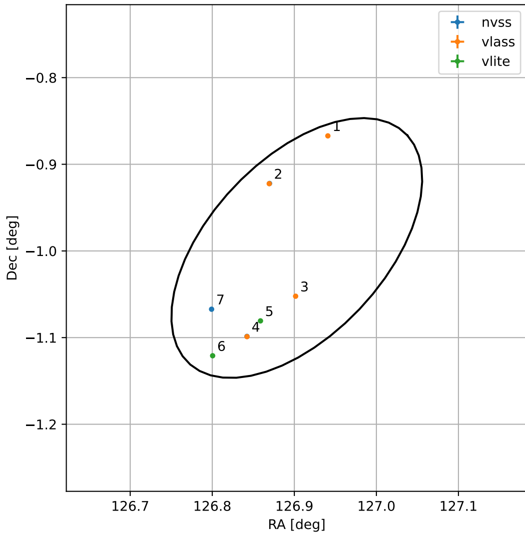
4FGL J0827.6-0059
