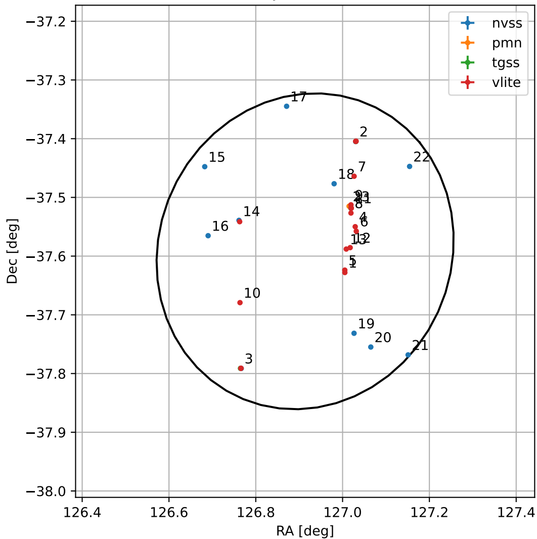
4FGL J0827.6-3735
