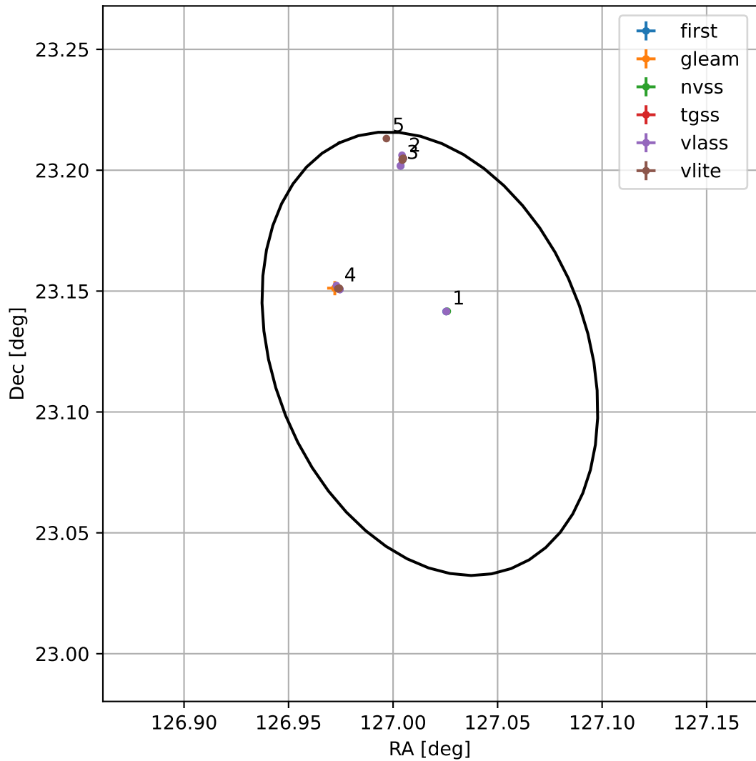
4FGL J0828.0+2307
