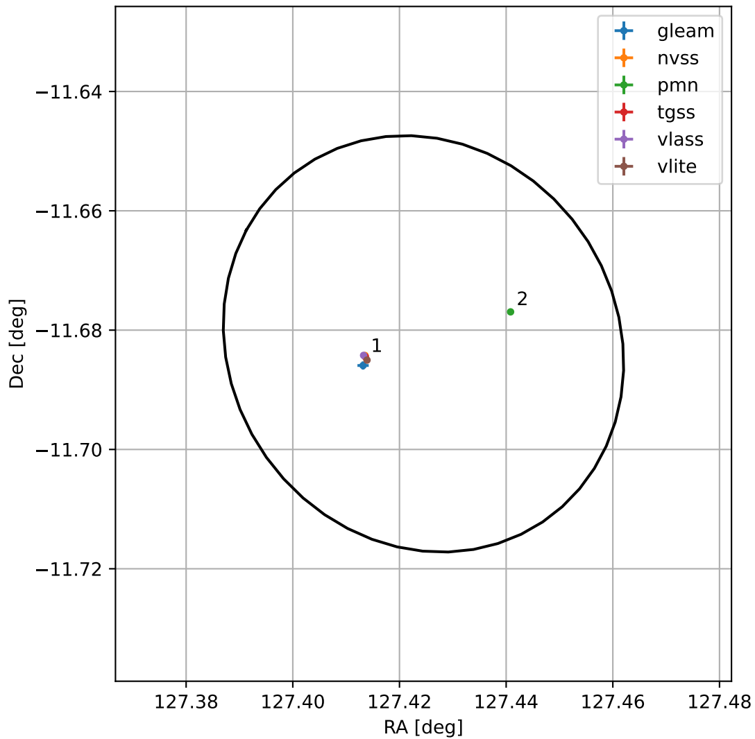
4FGL J0829.6-1140
