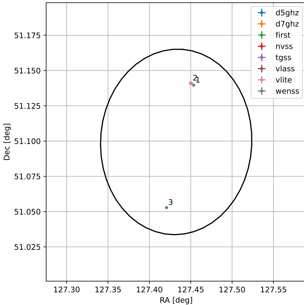
4FGL J0829.7+5105
