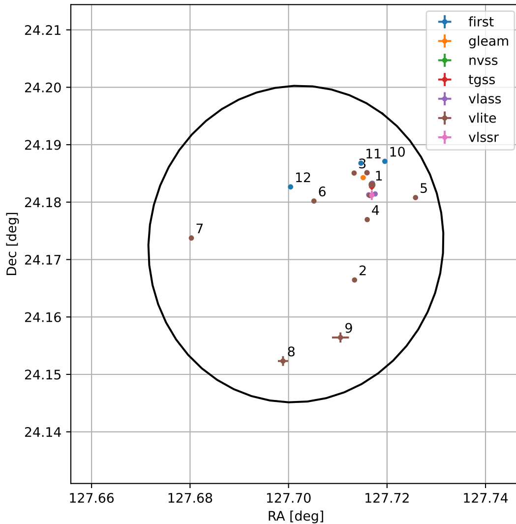
4FGL J0830.8+2410
