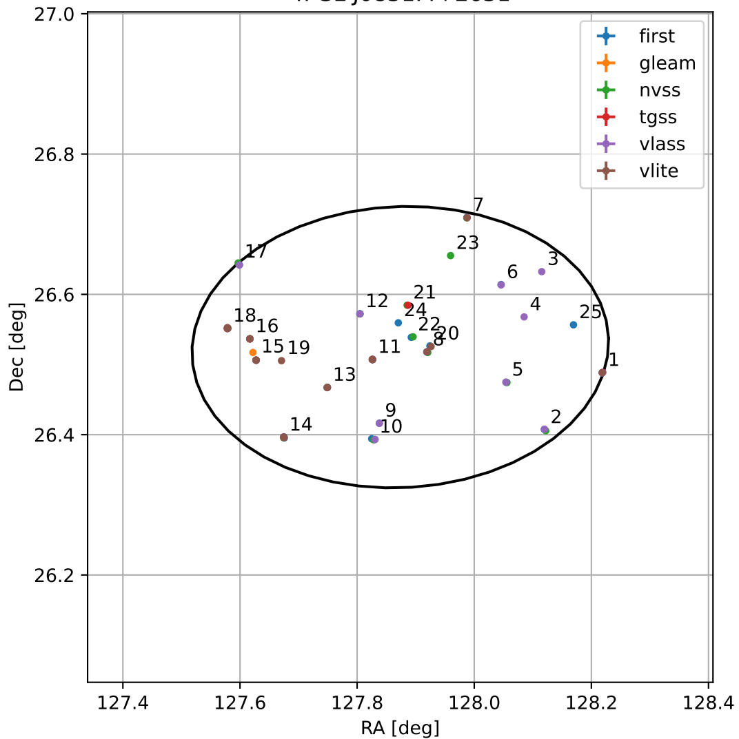
4FGL J0831.4+2631
