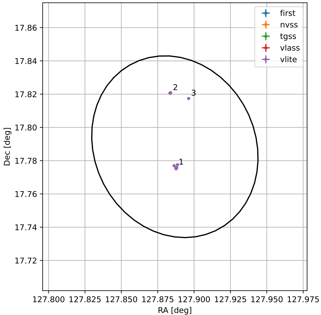
4FGL J0831.5+1747
