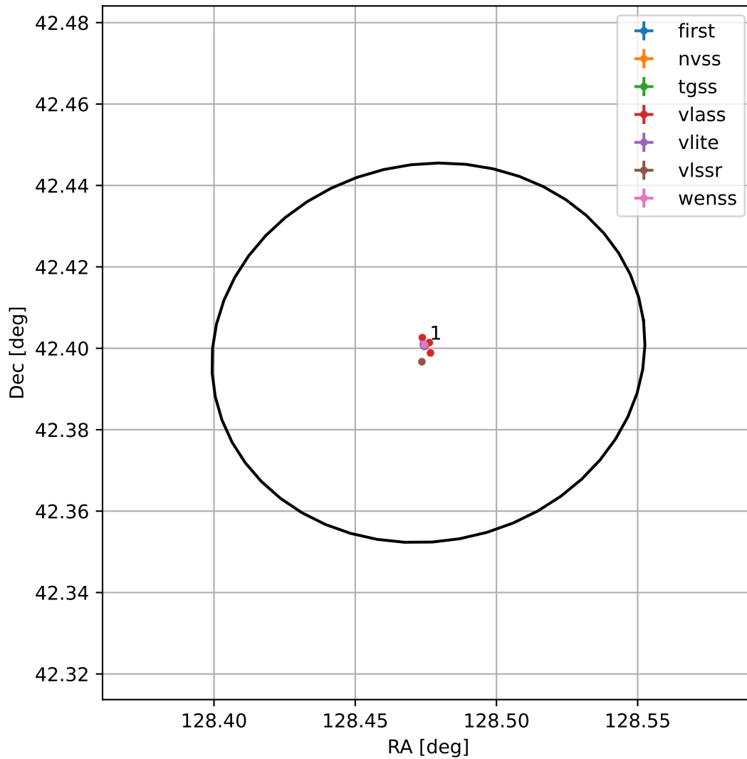
4FGL J0833.9+4223
