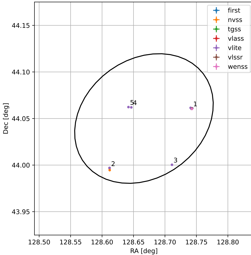
4FGL J0834.6+4402
