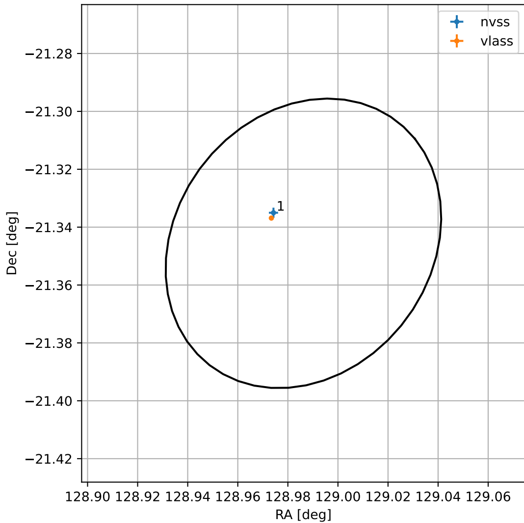
4FGL J0835.9-2120
