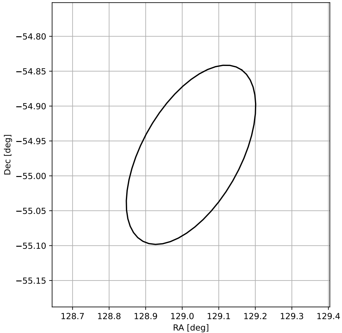
4FGL J0836.0-5458
