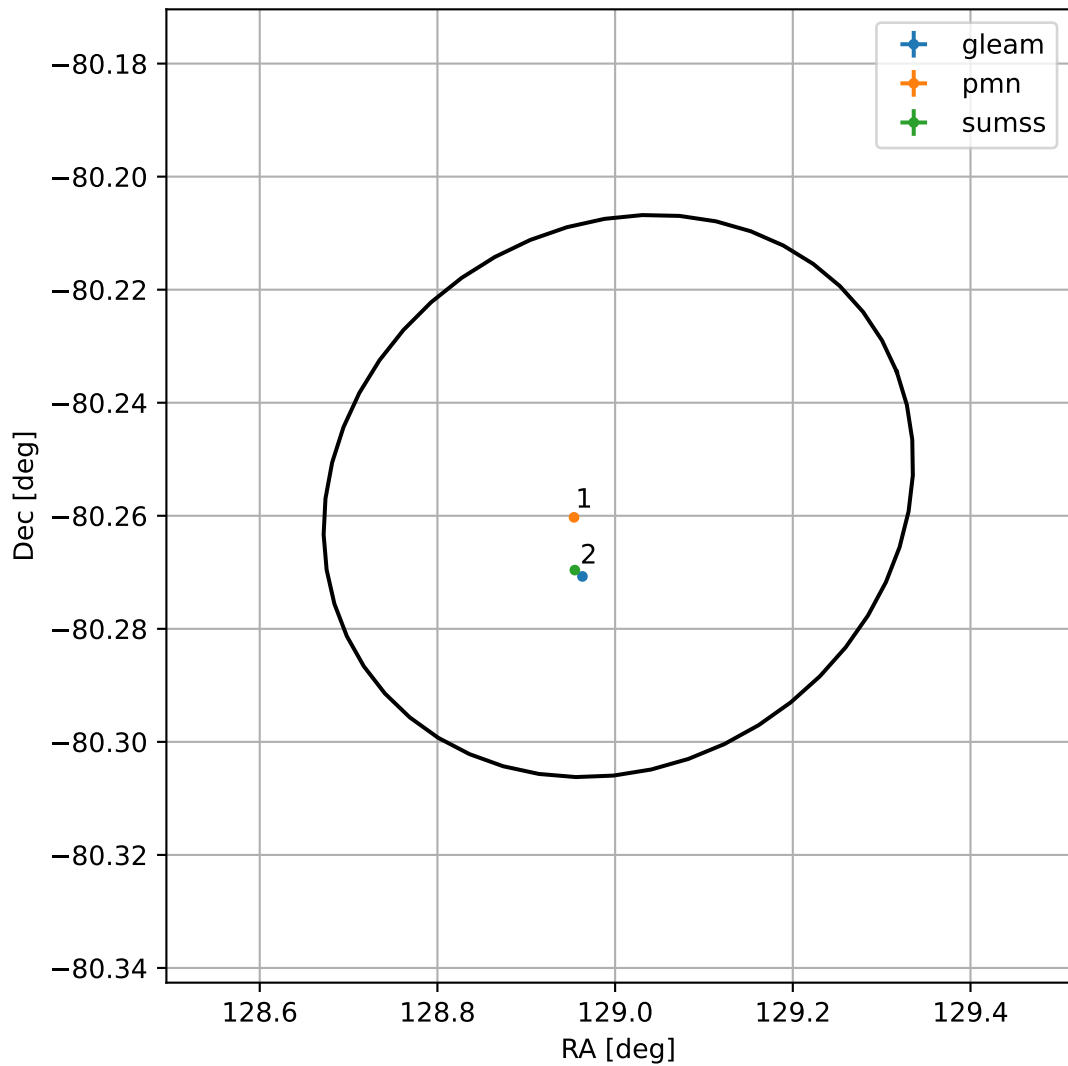
4FGL J0836.0-8015
