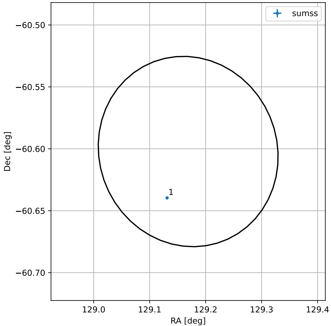
4FGL J0836.6-6036
