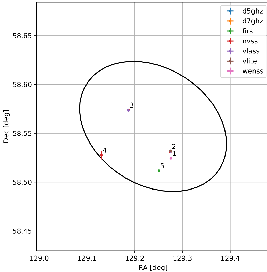
4FGL J0836.9+5833
