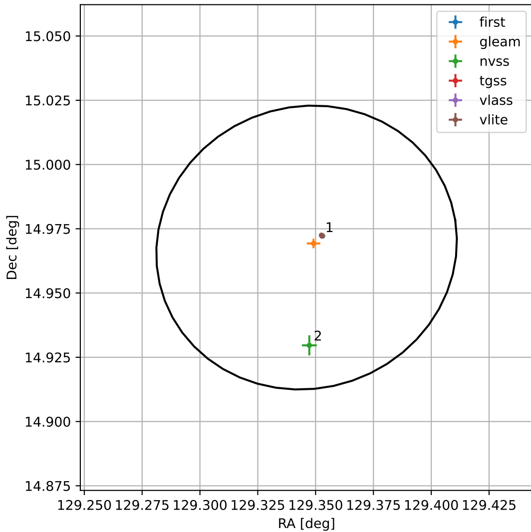
4FGL J0837.3+1458
