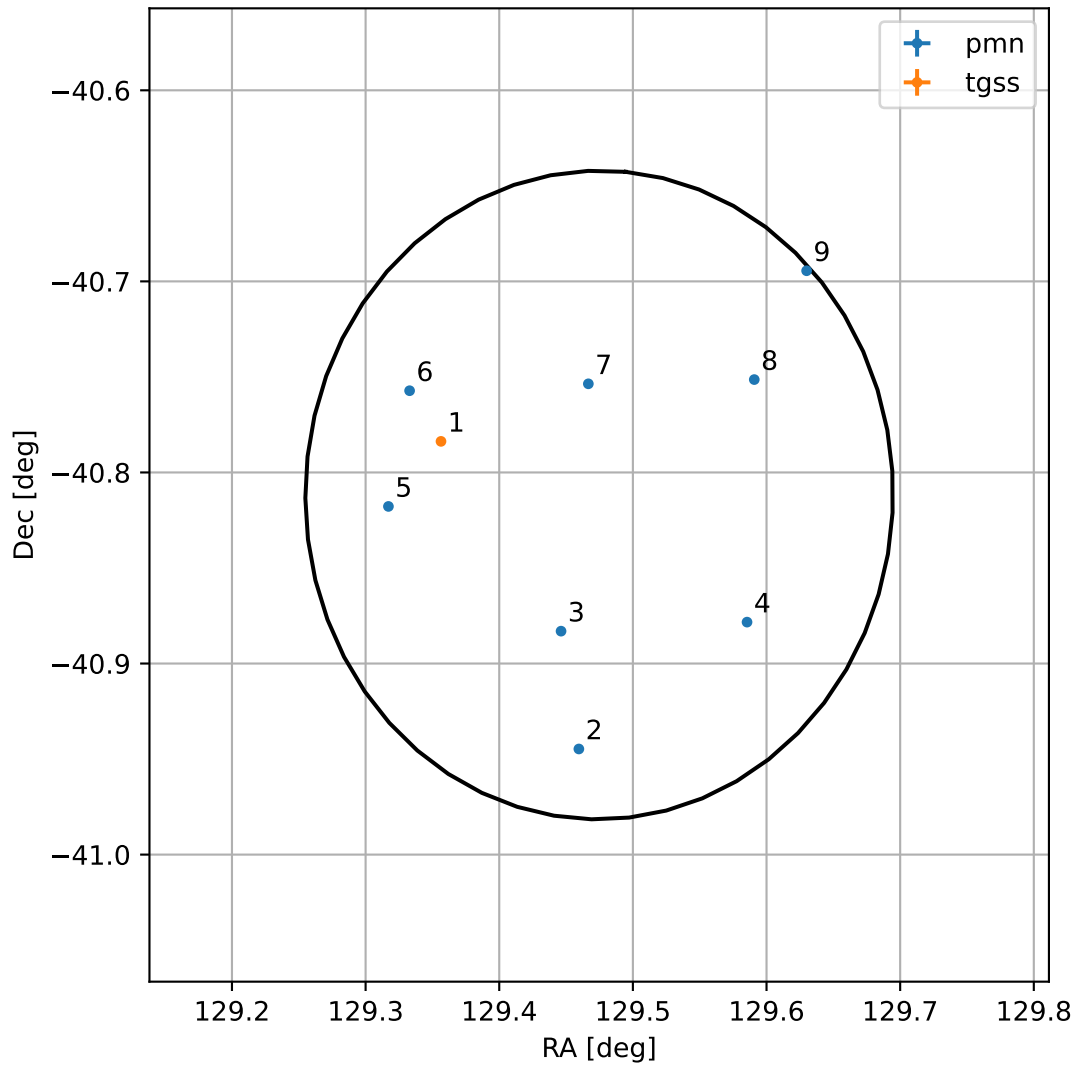
4FGL J0837.8-4048
