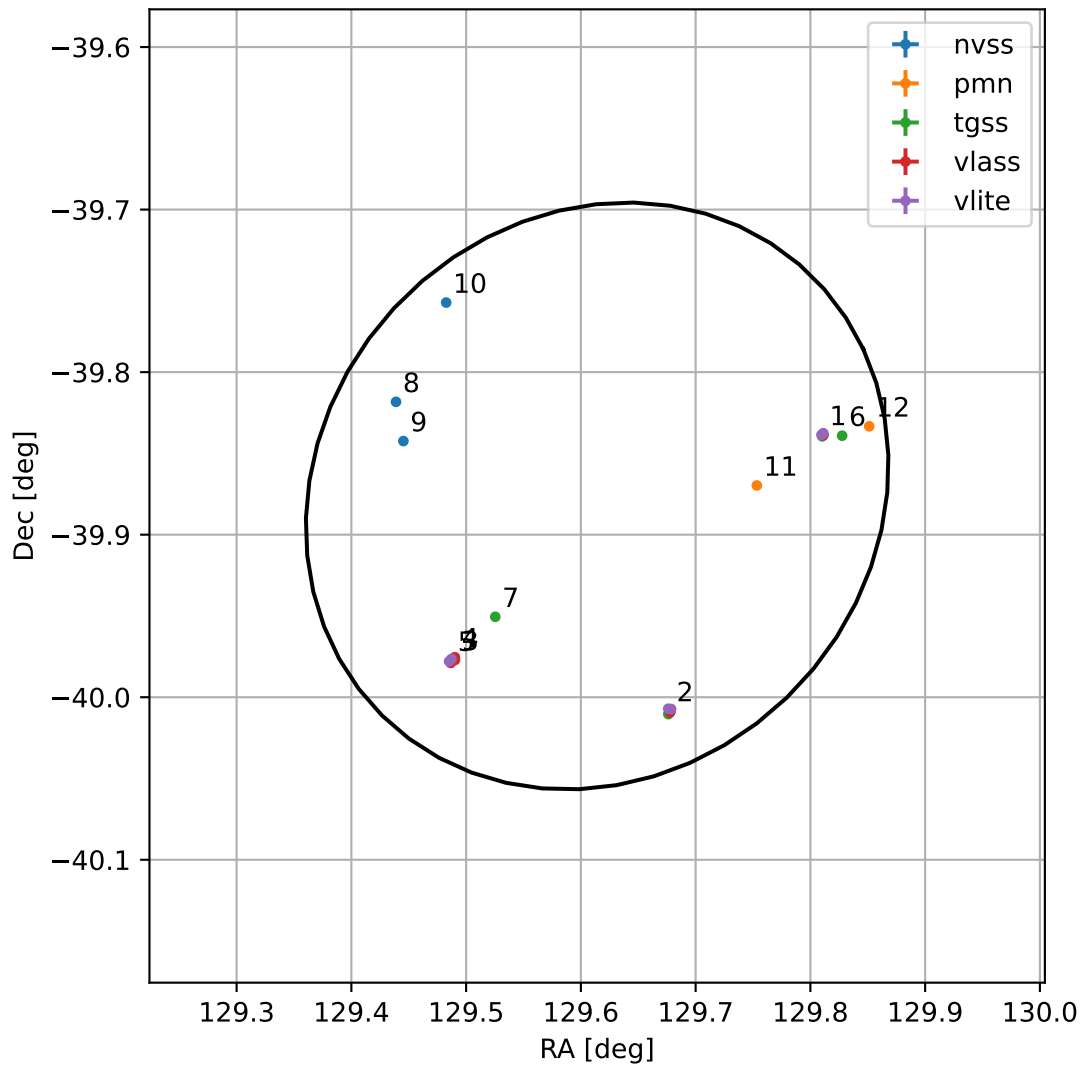
4FGL J0838.4-3952
