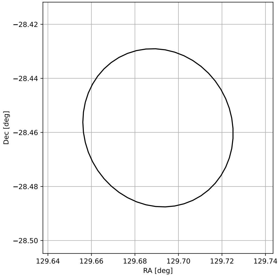
4FGL J0838.7-2827
