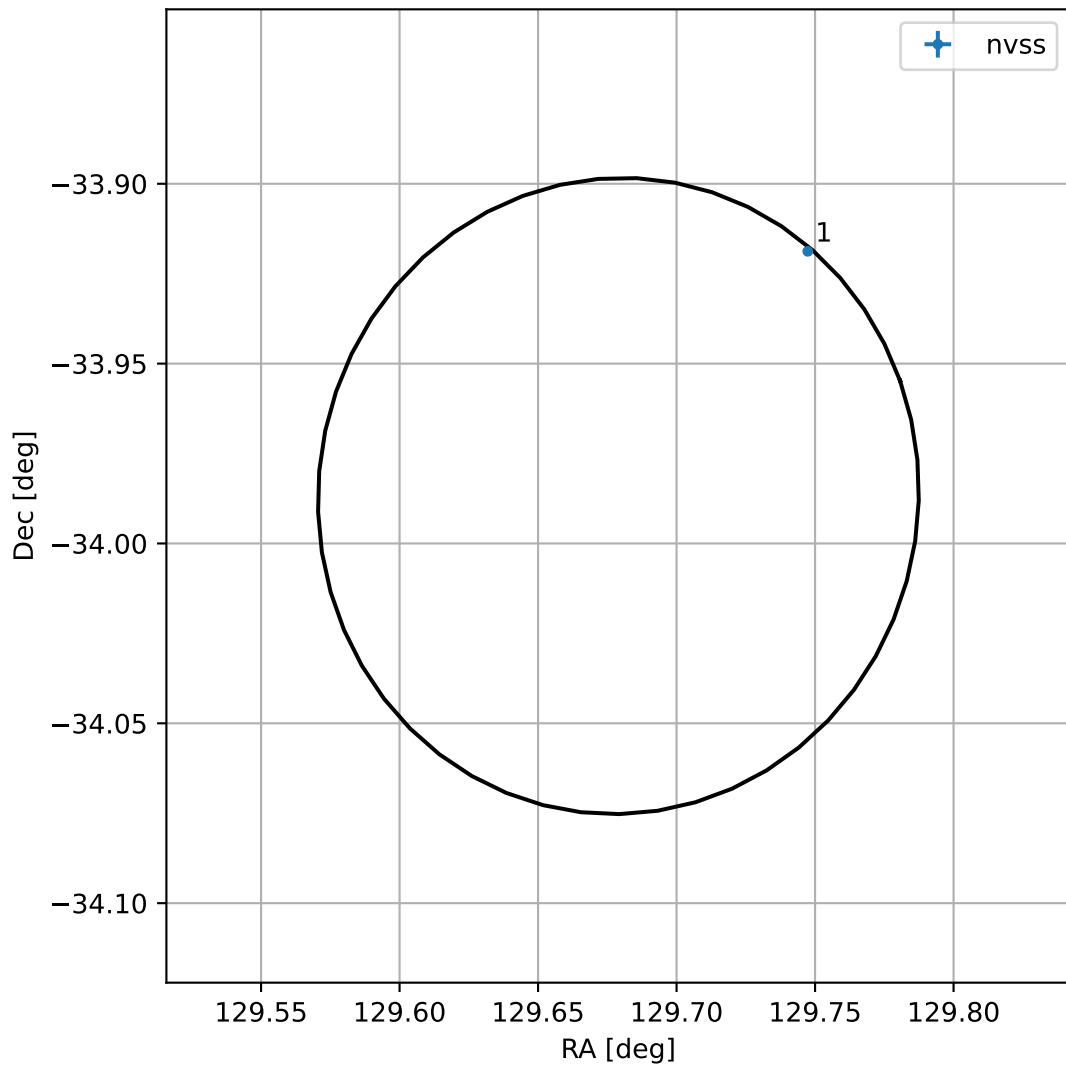
4FGL J0838.7-3359
