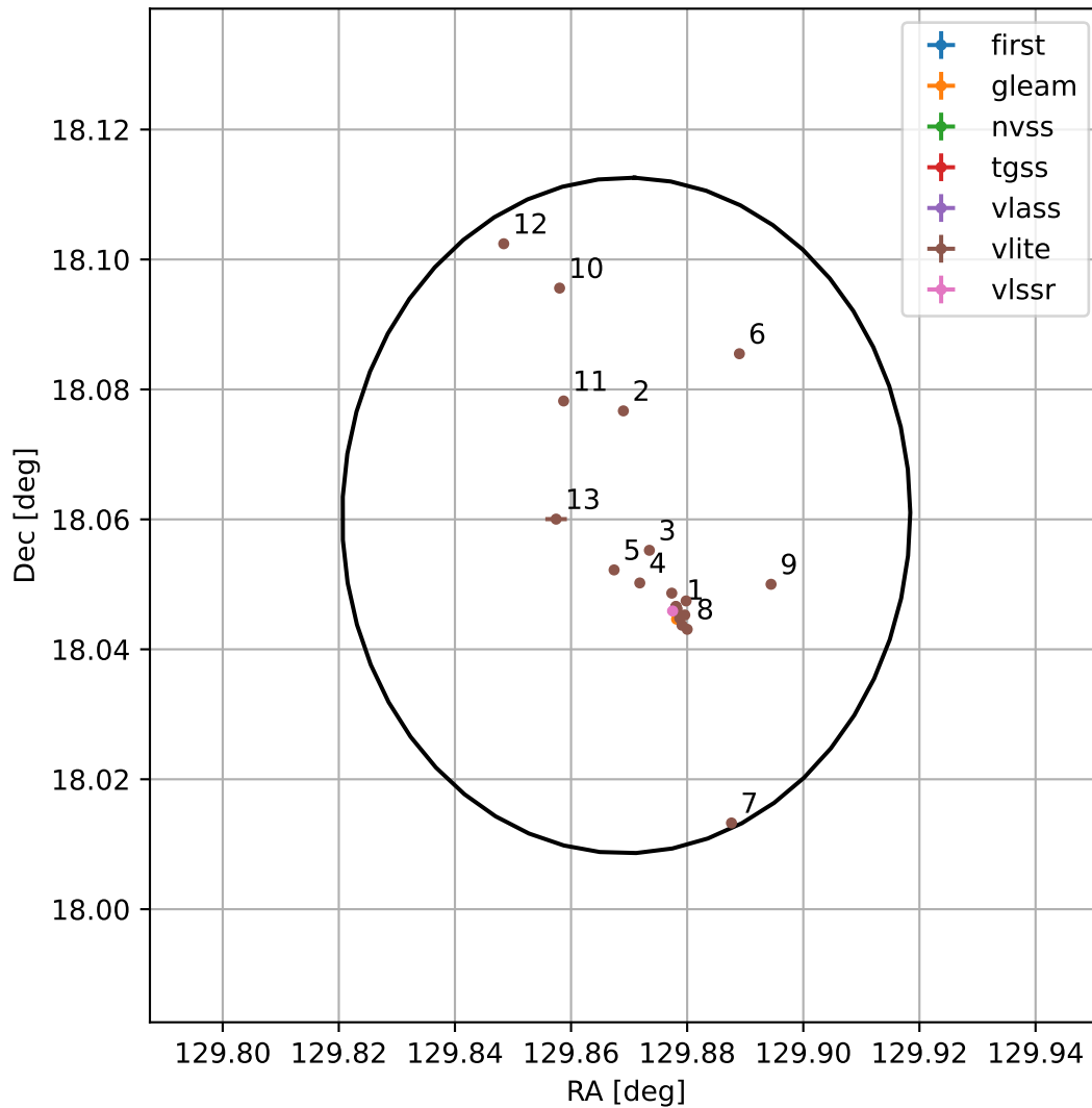
4FGL J0839.4+1803
