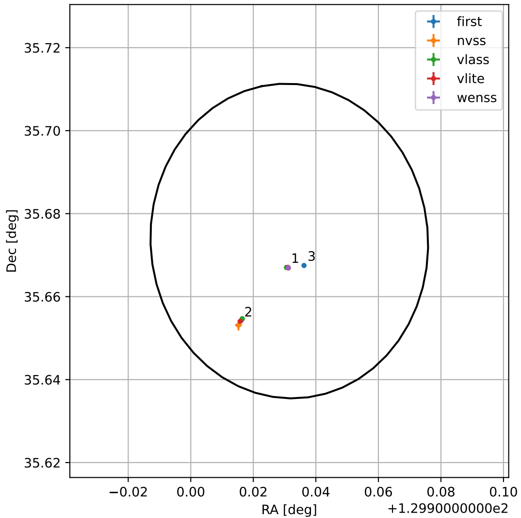
4FGL J0839.7+3540
