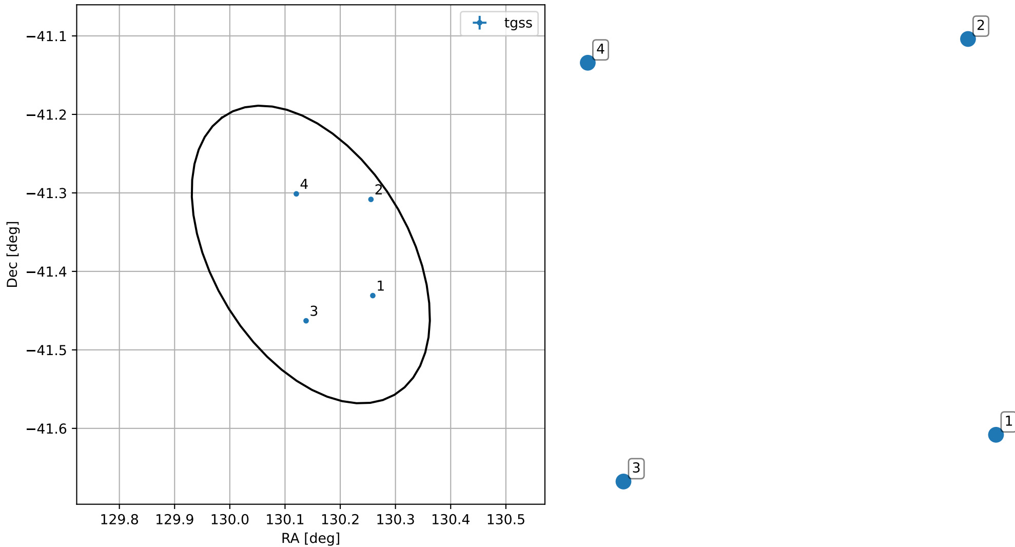
4FGL J0840.5-4122
