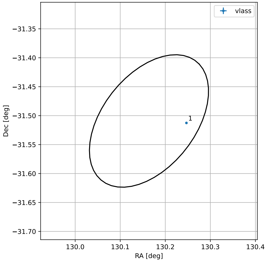
4FGL J0840.6-3130
