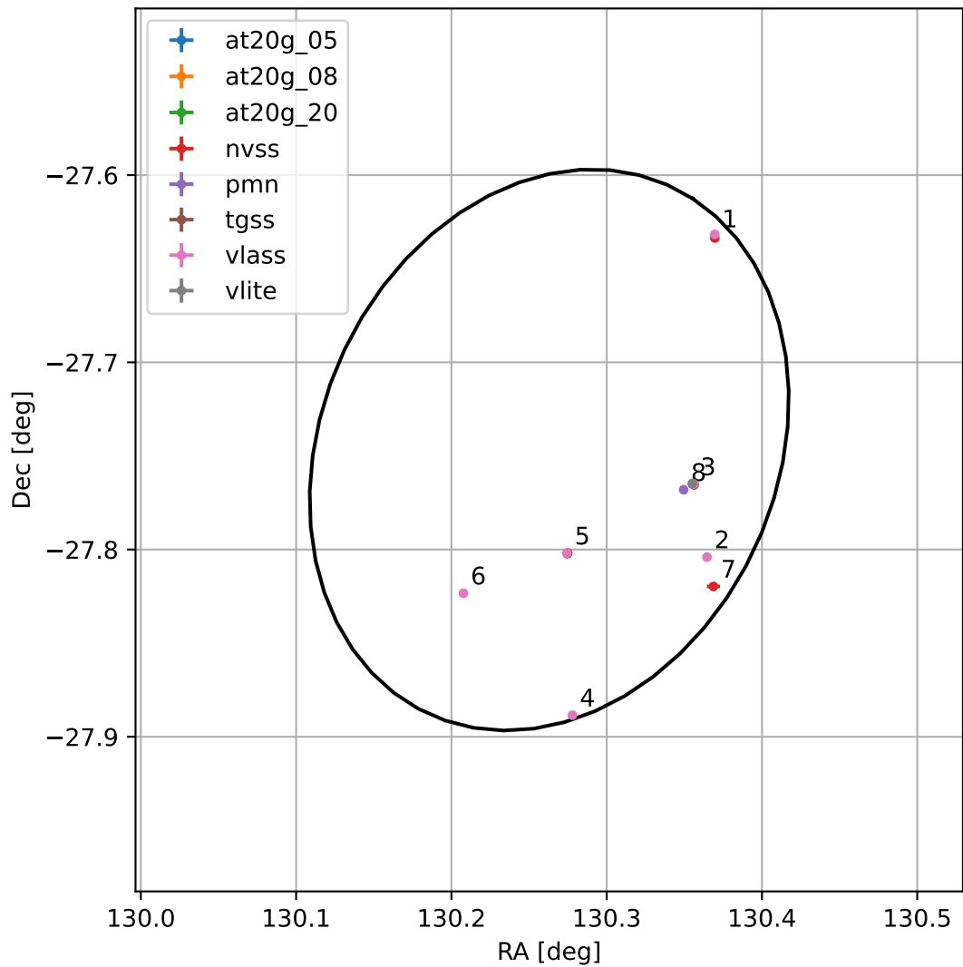
4FGL J0841.0-2744
