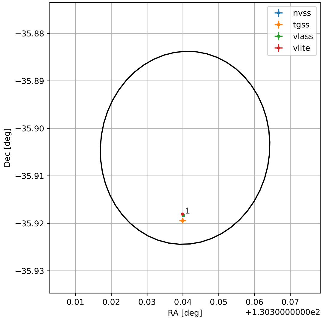
4FGL J0841.3-3554
