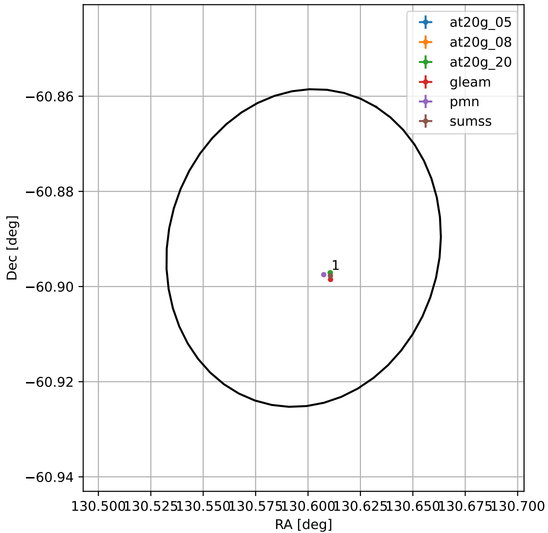
4FGL J0842.3-6053
