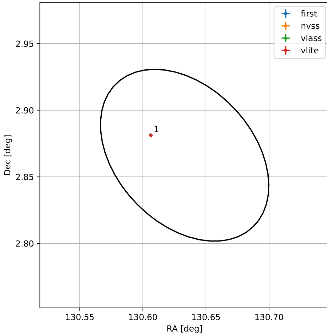
4FGL J0842.5+0251
