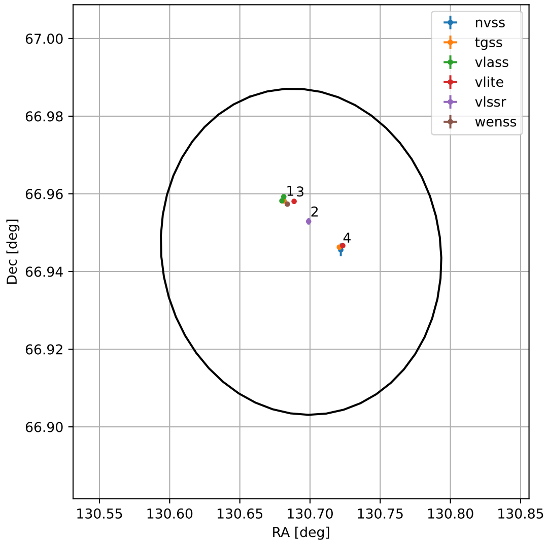
4FGL J0842.7+6656
