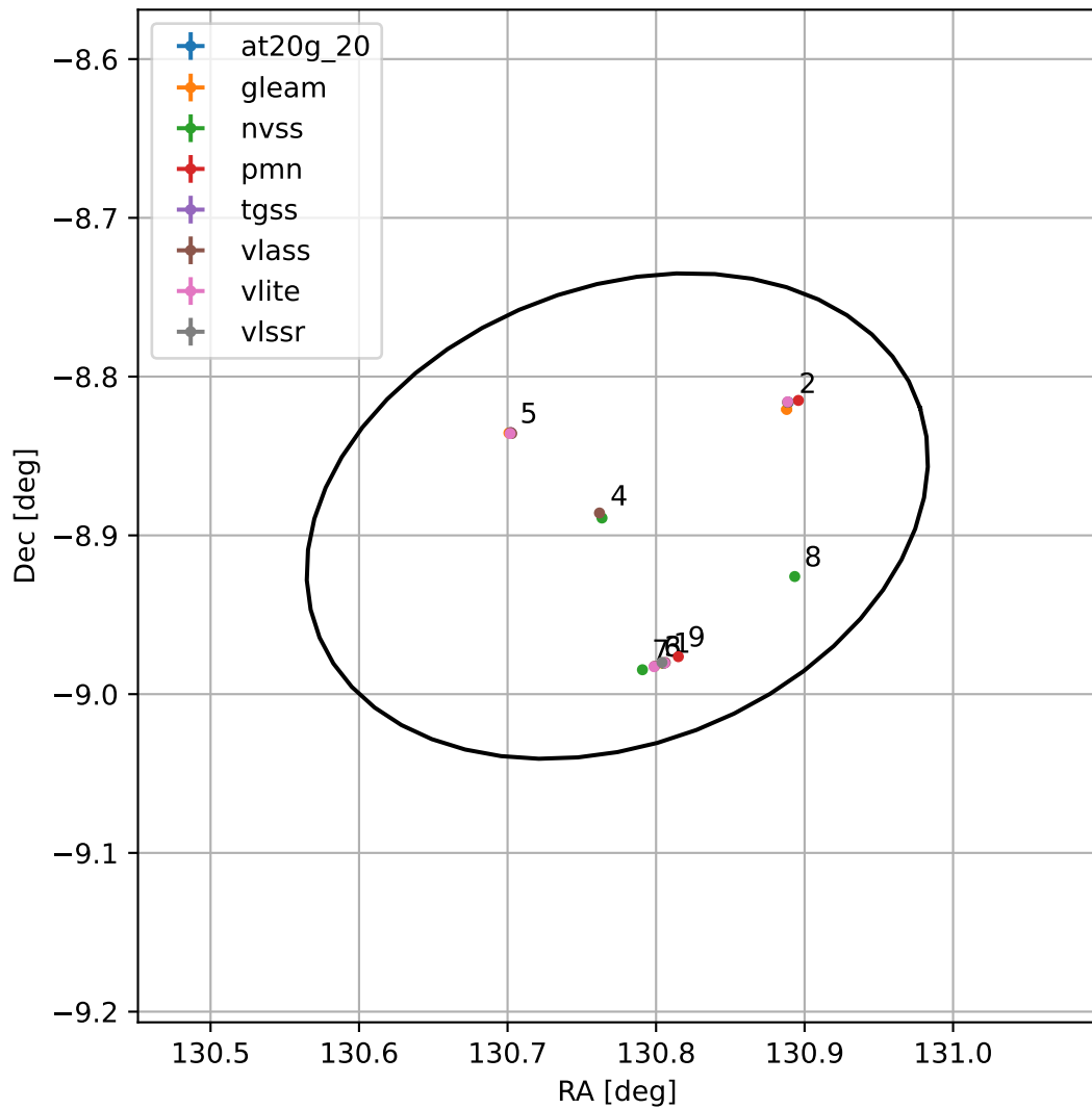
4FGL J0843.0-0853
