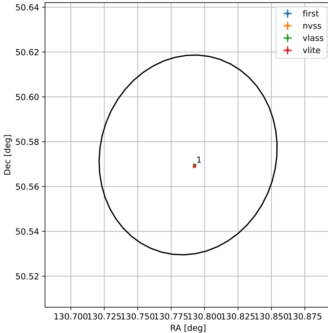
4FGL J0843.1+5034
