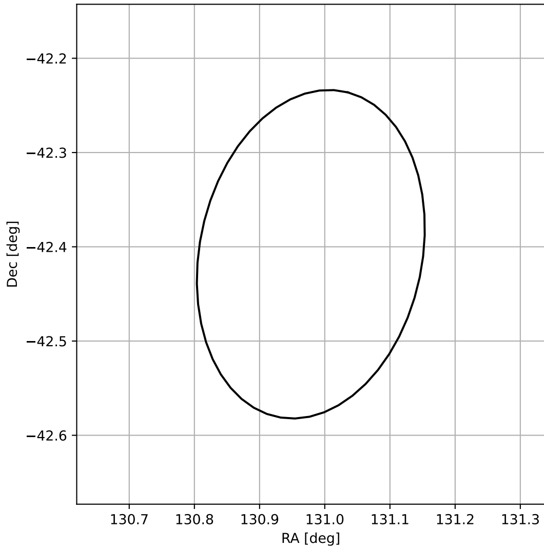
4FGL J0843.9-4224
