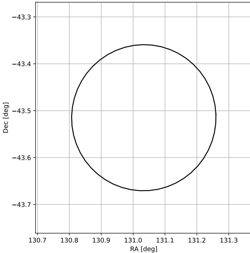
4FGL J0844.1-4330
