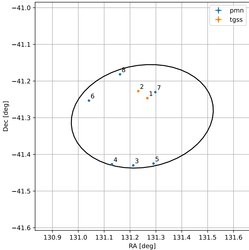
4FGL J0844.9-4117
