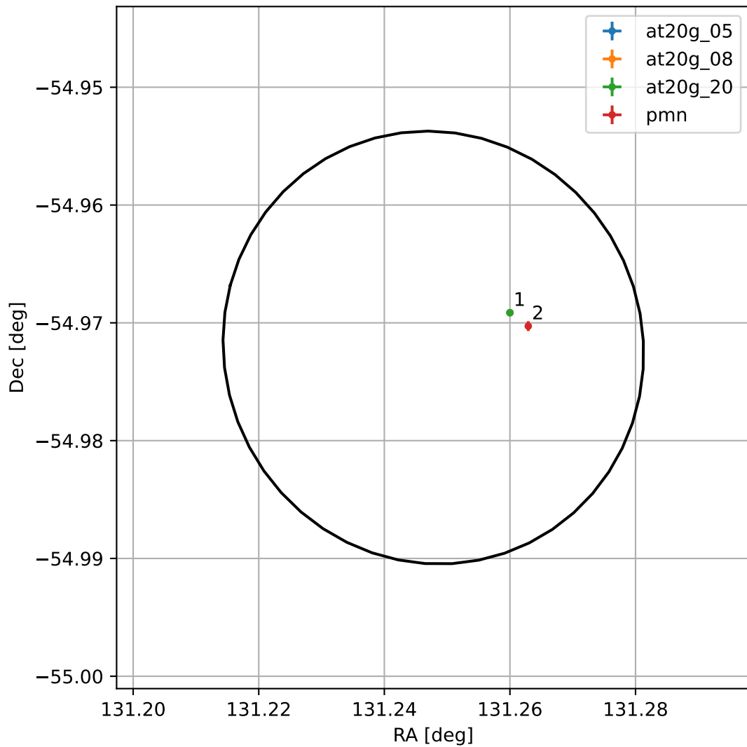
4FGL J0844.9-5458
