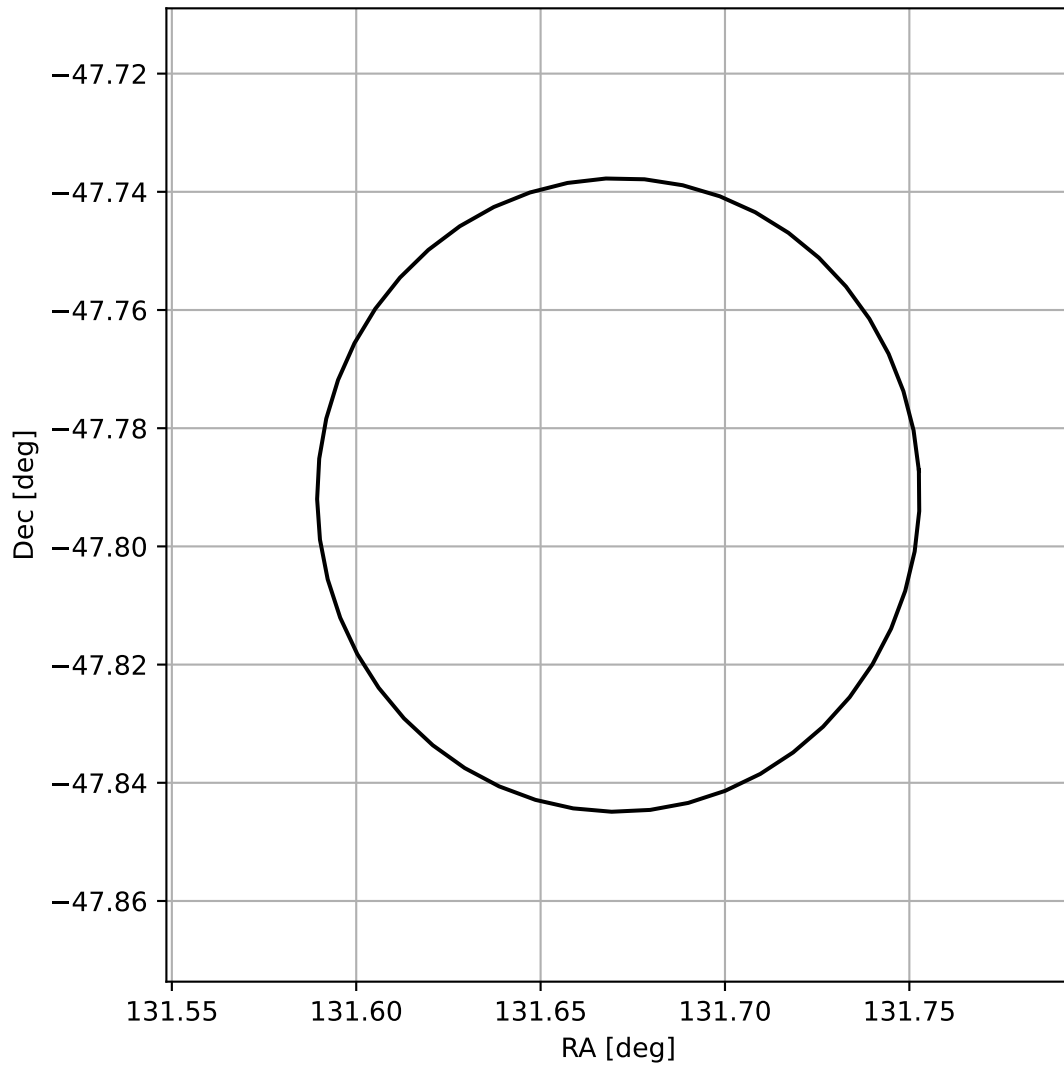
4FGL J0846.6-4747
