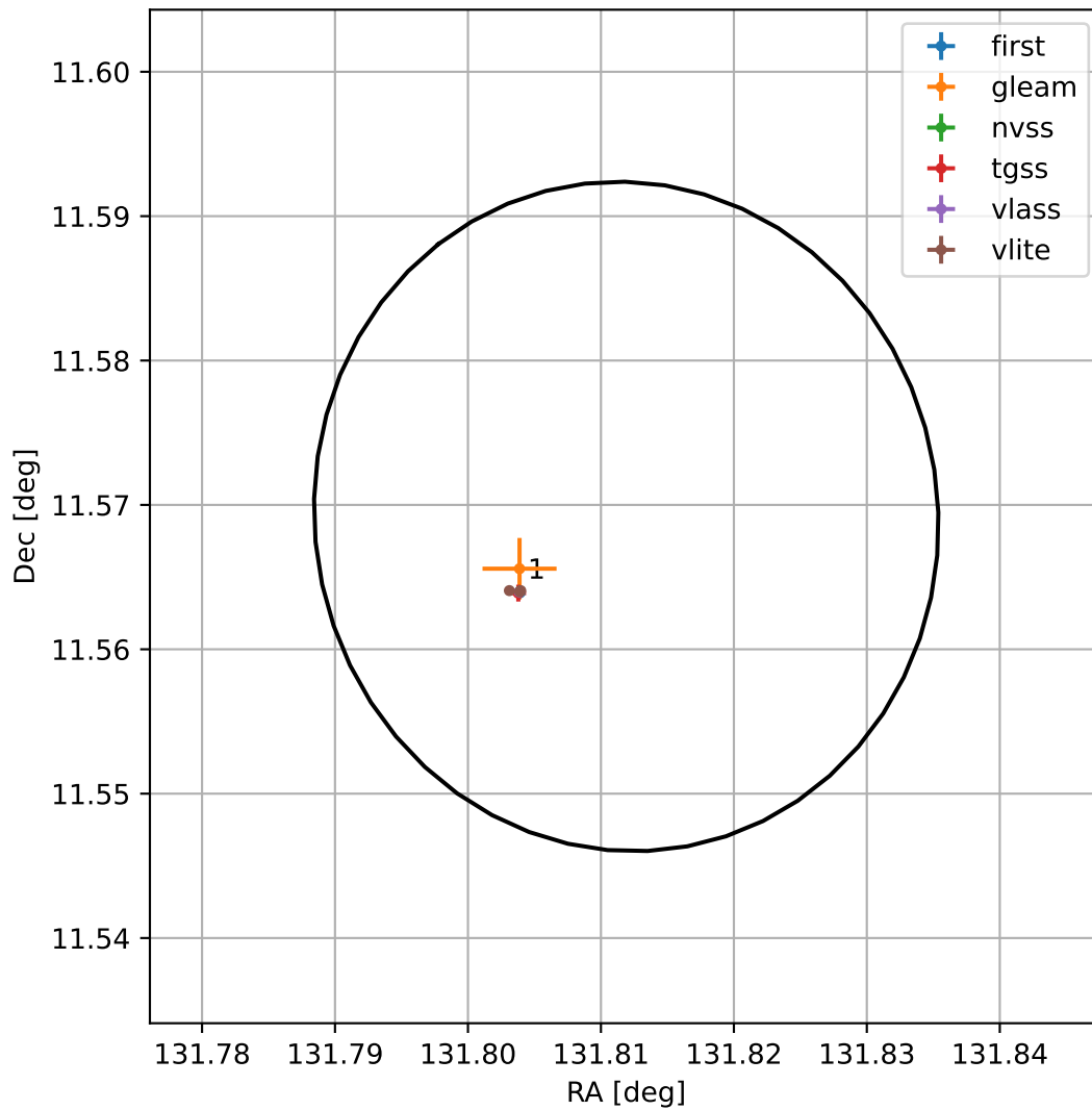
4FGL J0847.2+1134
