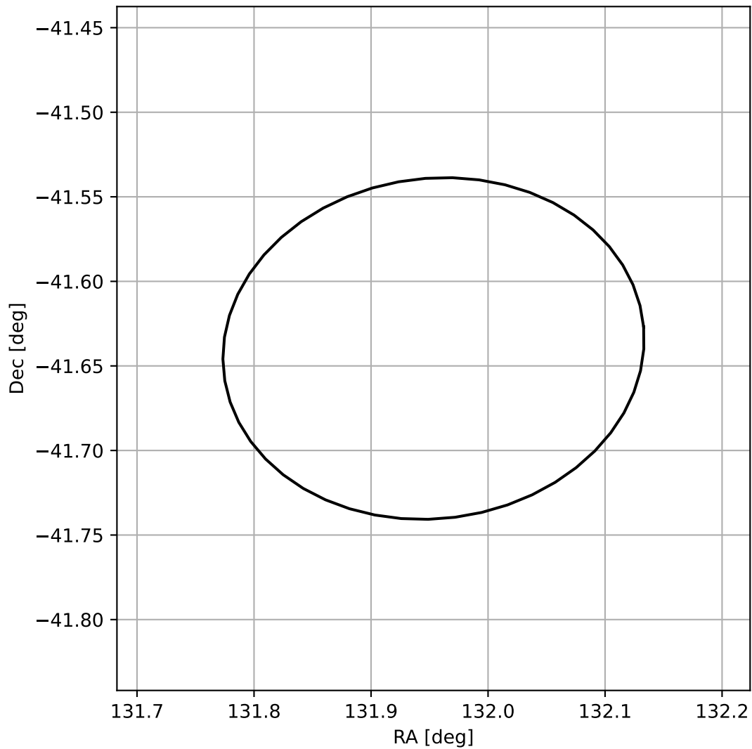
4FGL J0847.8-4138
