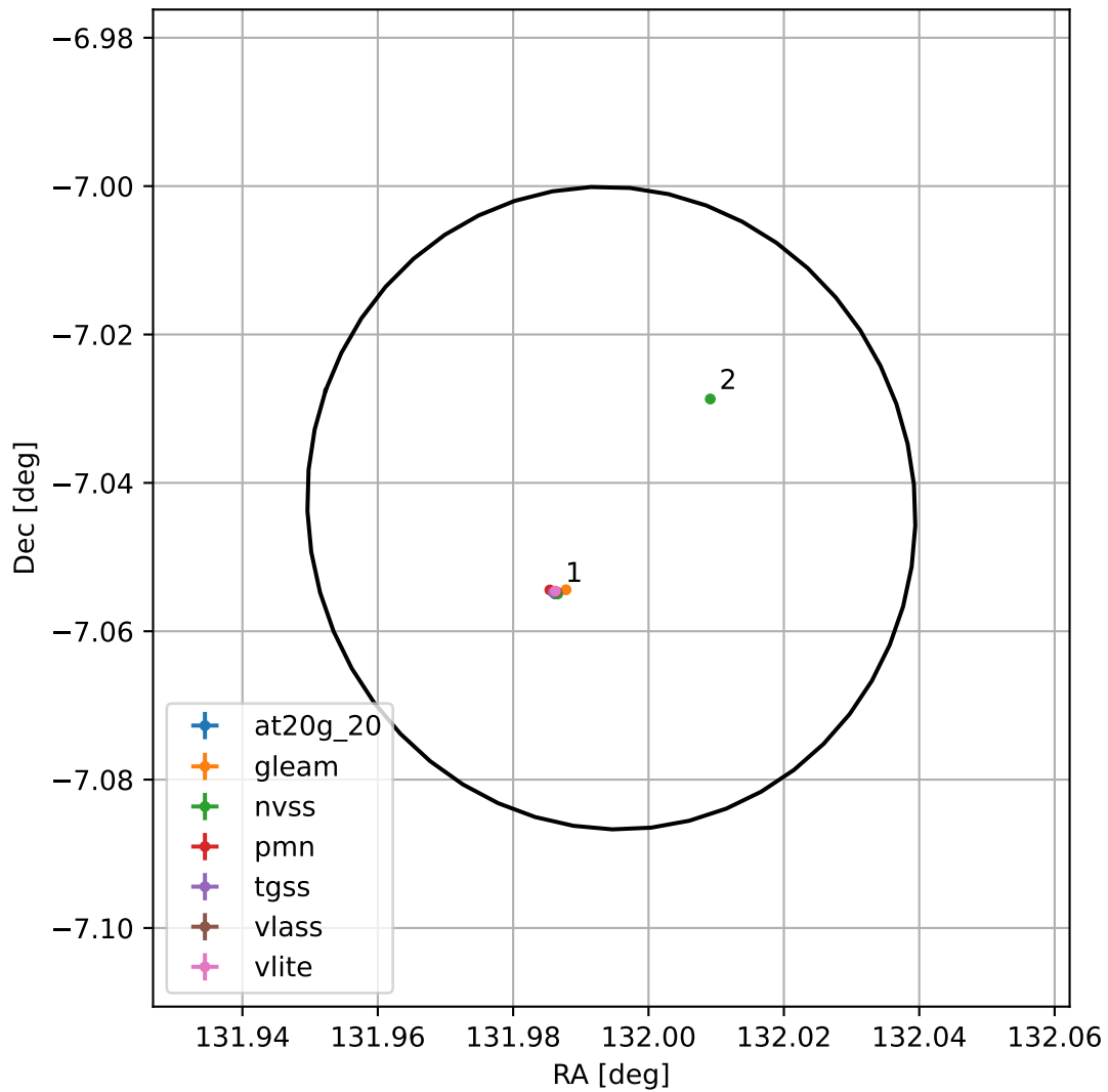
4FGL J0847.9-0702
