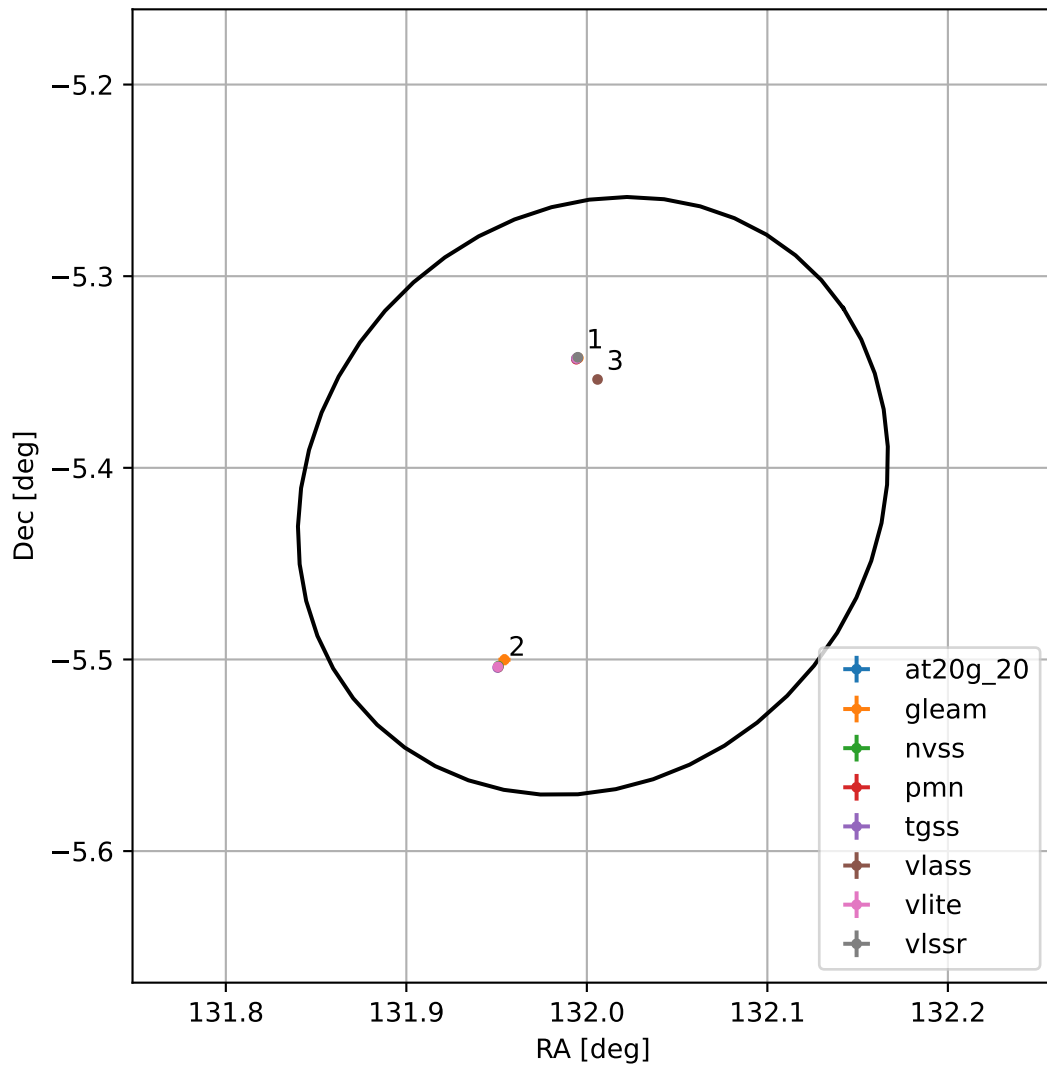
4FGL J0848.0-0524
