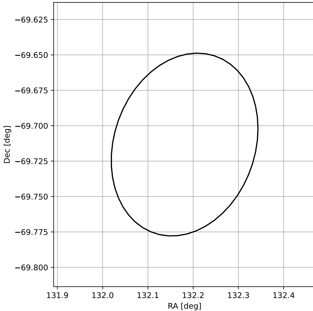
4FGL J0848.7-6942
