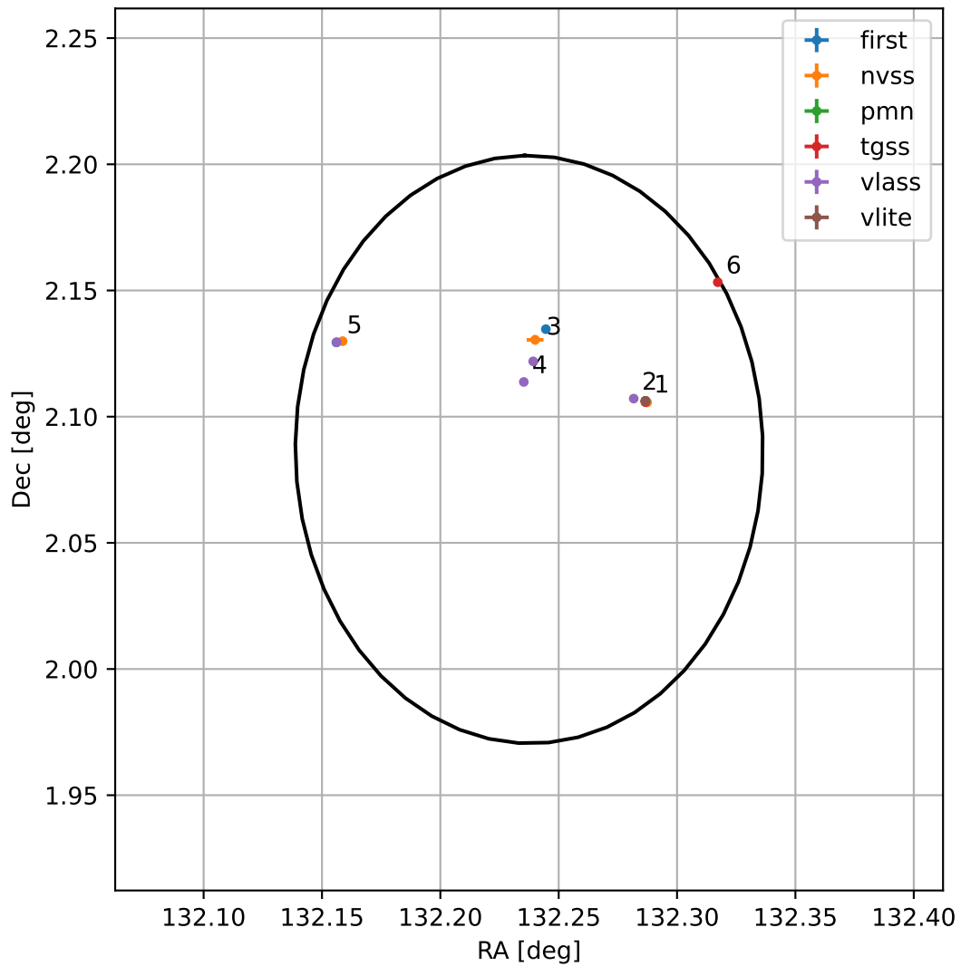
4FGL J0848.9+0205
