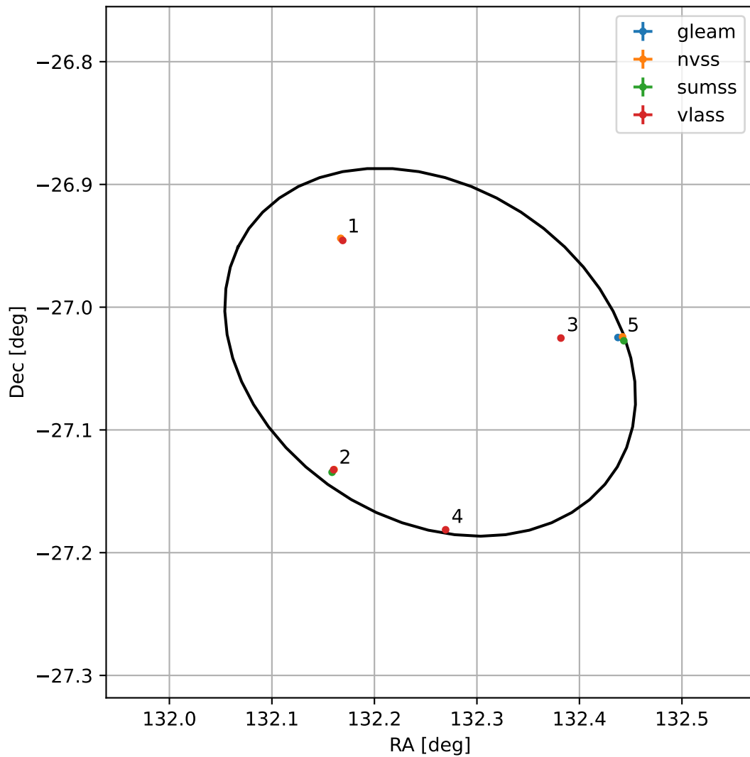
4FGL J0849.0-2702
