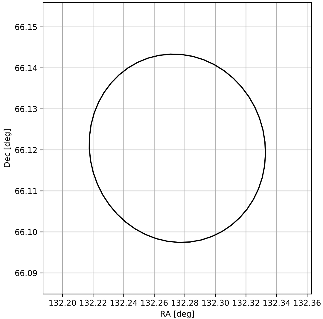
4FGL J0849.1+6607
