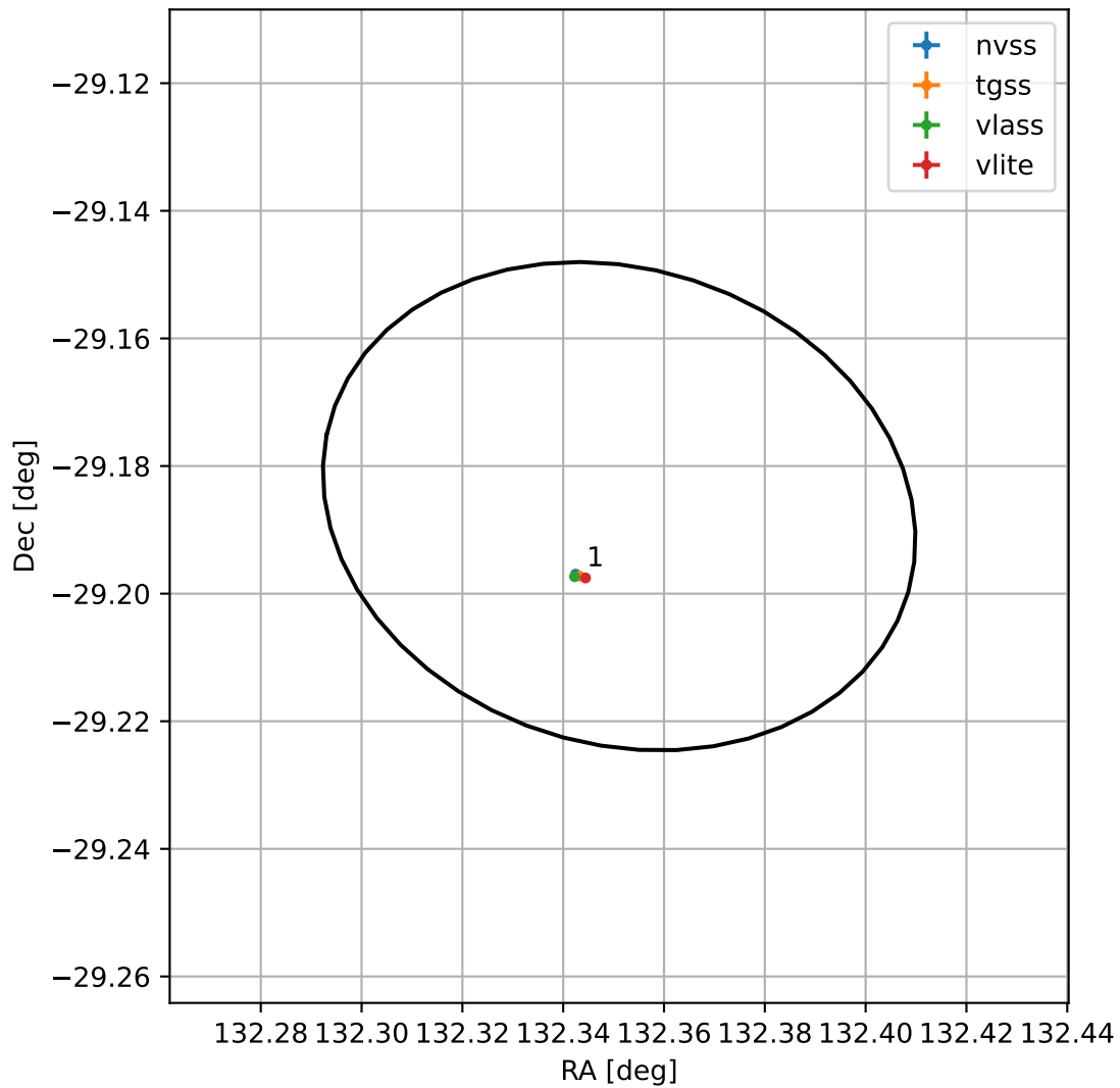
4FGL J0849.4-2911
