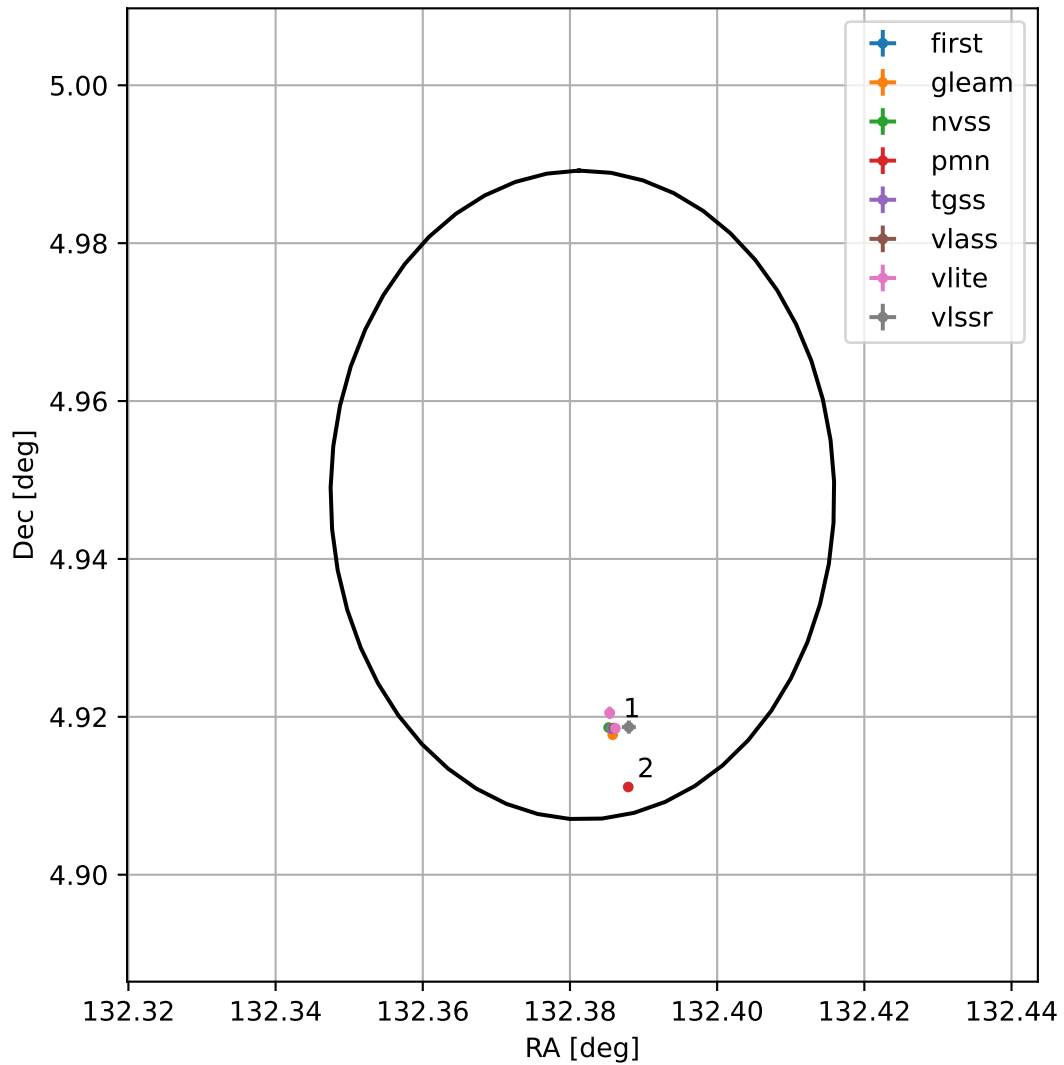
4FGL J0849.5+0456
